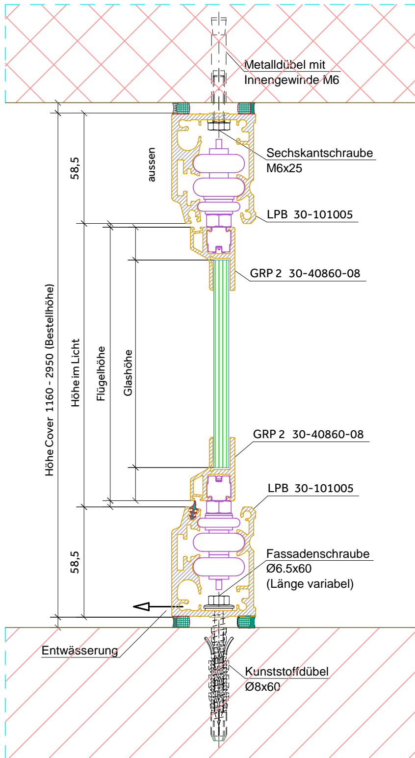
Bodendetail standard
