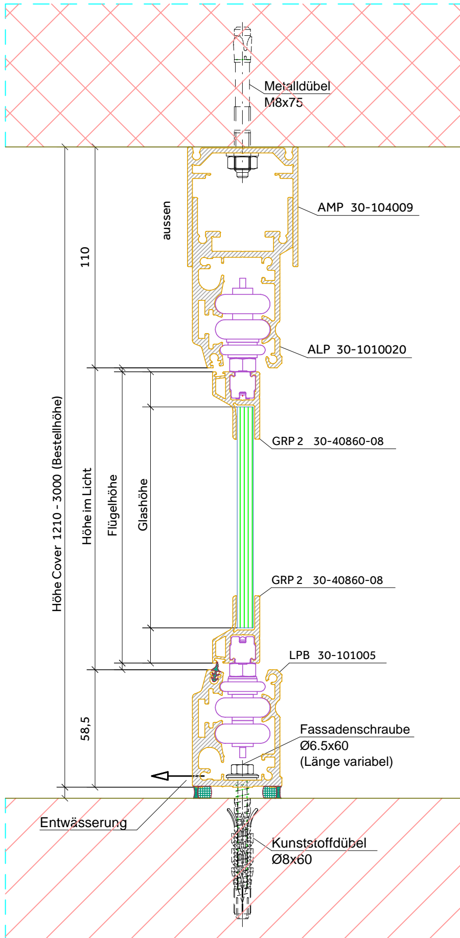
Bodendetail standard
